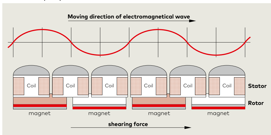
The functional principle of MAGNEO
